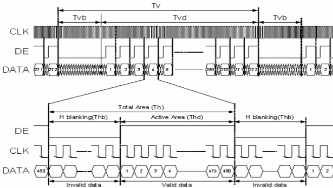
Parallel DE mode RGB input timing table
